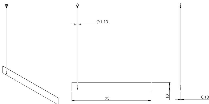
Antenna drawing. Above dimensions are given in millimeter.
